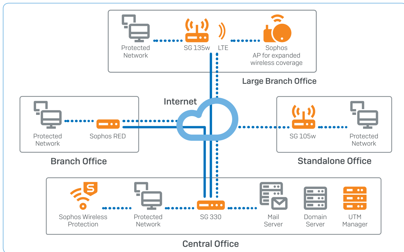
A typical deployment scenario using the SG 135w and SG 105w as part of a distributed organization.
